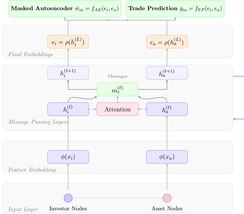
Figure 1: Model architecture
