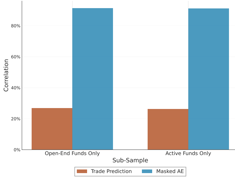
(a) Validation set performance, by subsample
