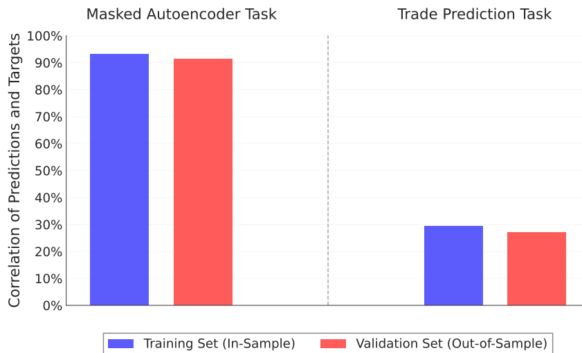
Figure 2: Performance metrics
